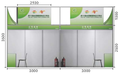
展位侧面图 Side elevation of booth
