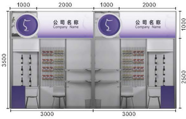
展位侧面图 Side elevation of booth
